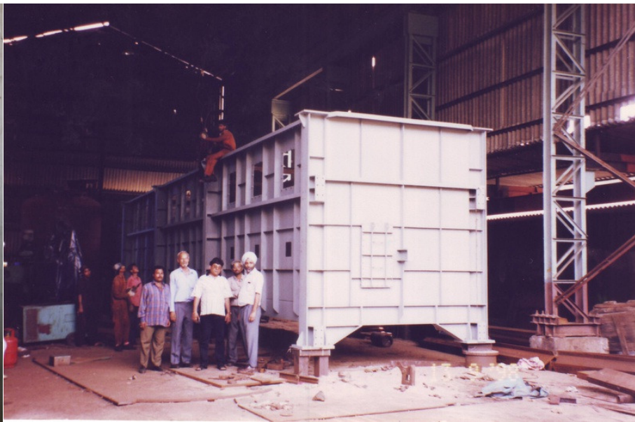
< Furnace made for HPCL.
